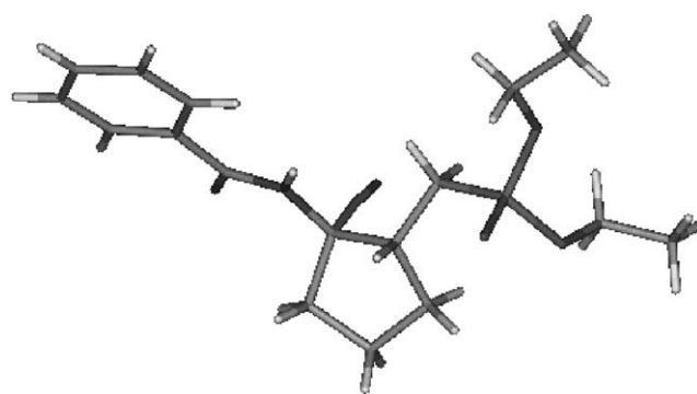
Figure 1. X-ray crystal structure of 21 .
